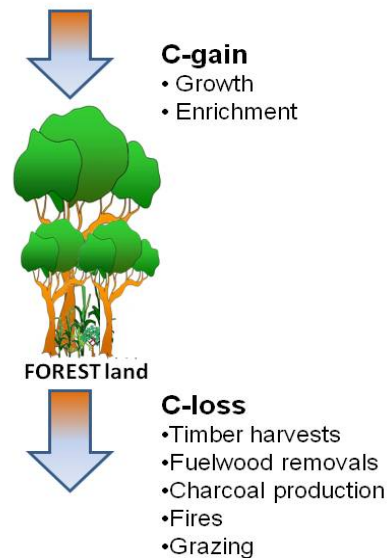
Figure 5.2. Comparison of stock-difference and gain-loss methods
